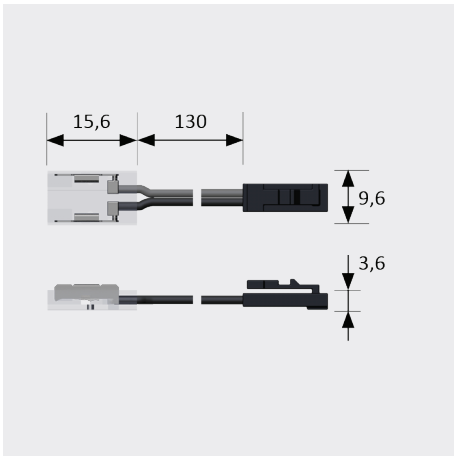
Feeder 130 mm for sections Order no. 36 373 42
