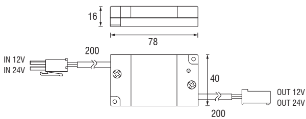
Centralina Control Unit / Relaisstation
